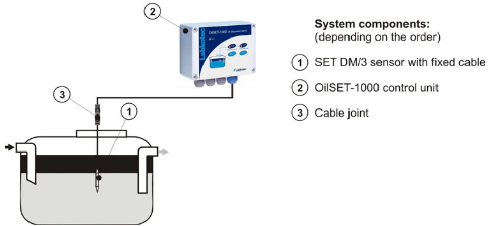
Figure 1. Oil separator alarm system
