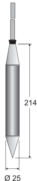
Figure 9. Dimensional drawing of SET DM/3 sensor
